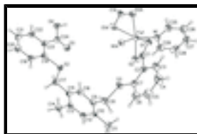
Fig. 1. Molecular structure showing 35% probability displacement ellipsoids. The atoms marked with A are derived from the reference atoms by the symmetry transformation of (-x, y, z) .
